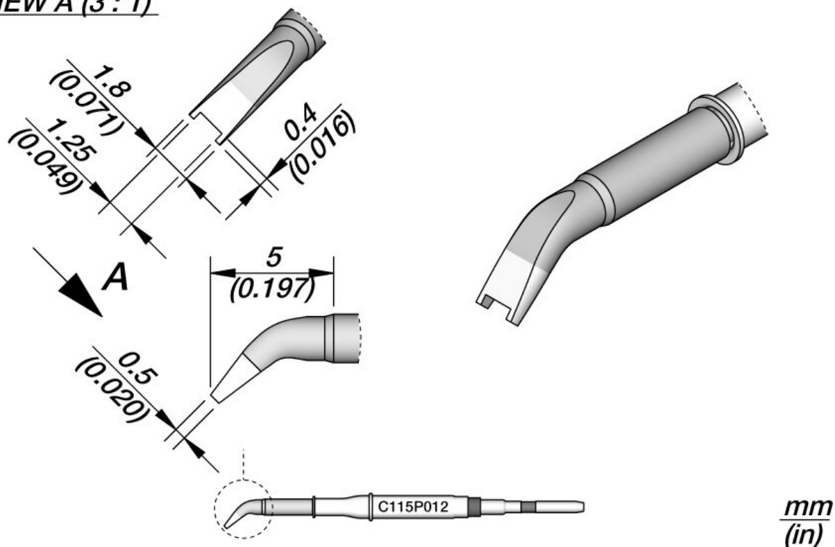
VIEW A (3 : 1)
